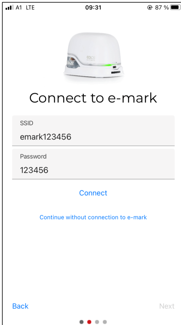
Fig. 33: Software wizard – Connection to e-mark
