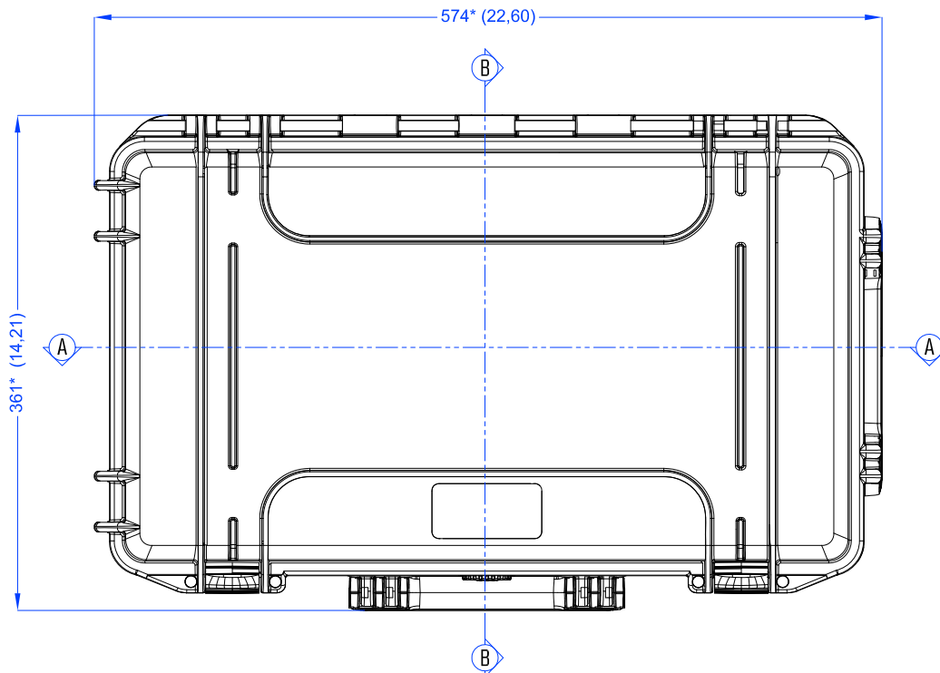
Vista Coperchio Lid View
